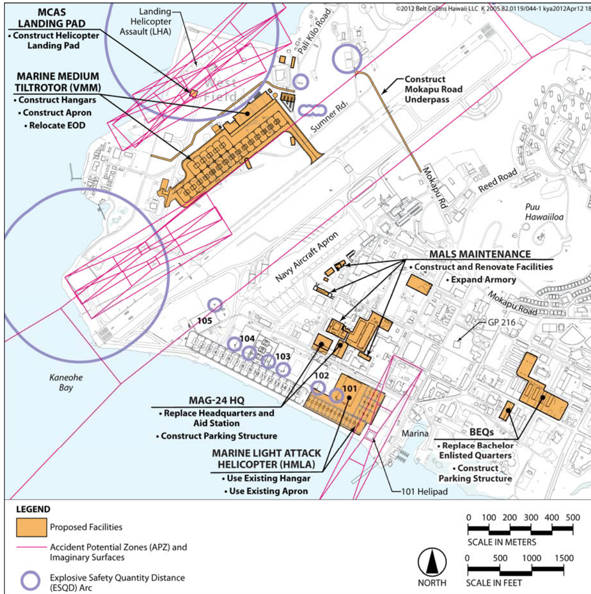
Figure ES-3. Alternative B – Overview, MCB Hawaii Kaneohe Bay
