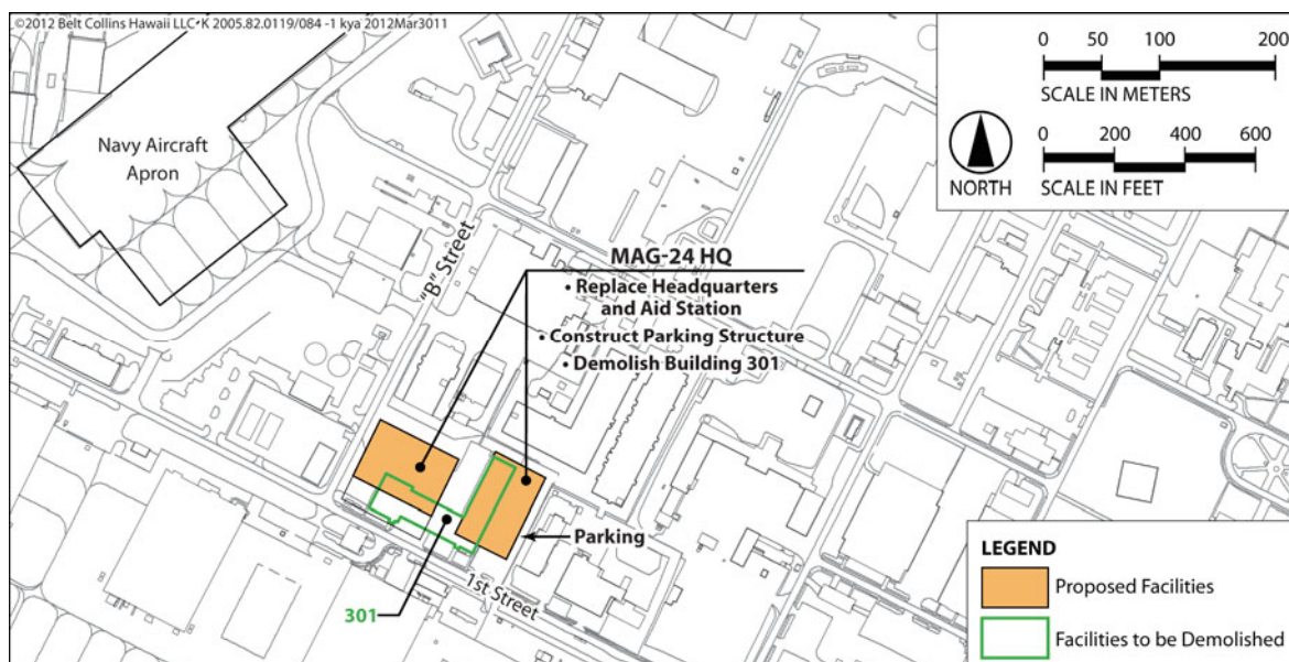
Figure 2-6. Alternative A - MAG-24 Headquarters, MCB Hawaii Kaneohe Bay
