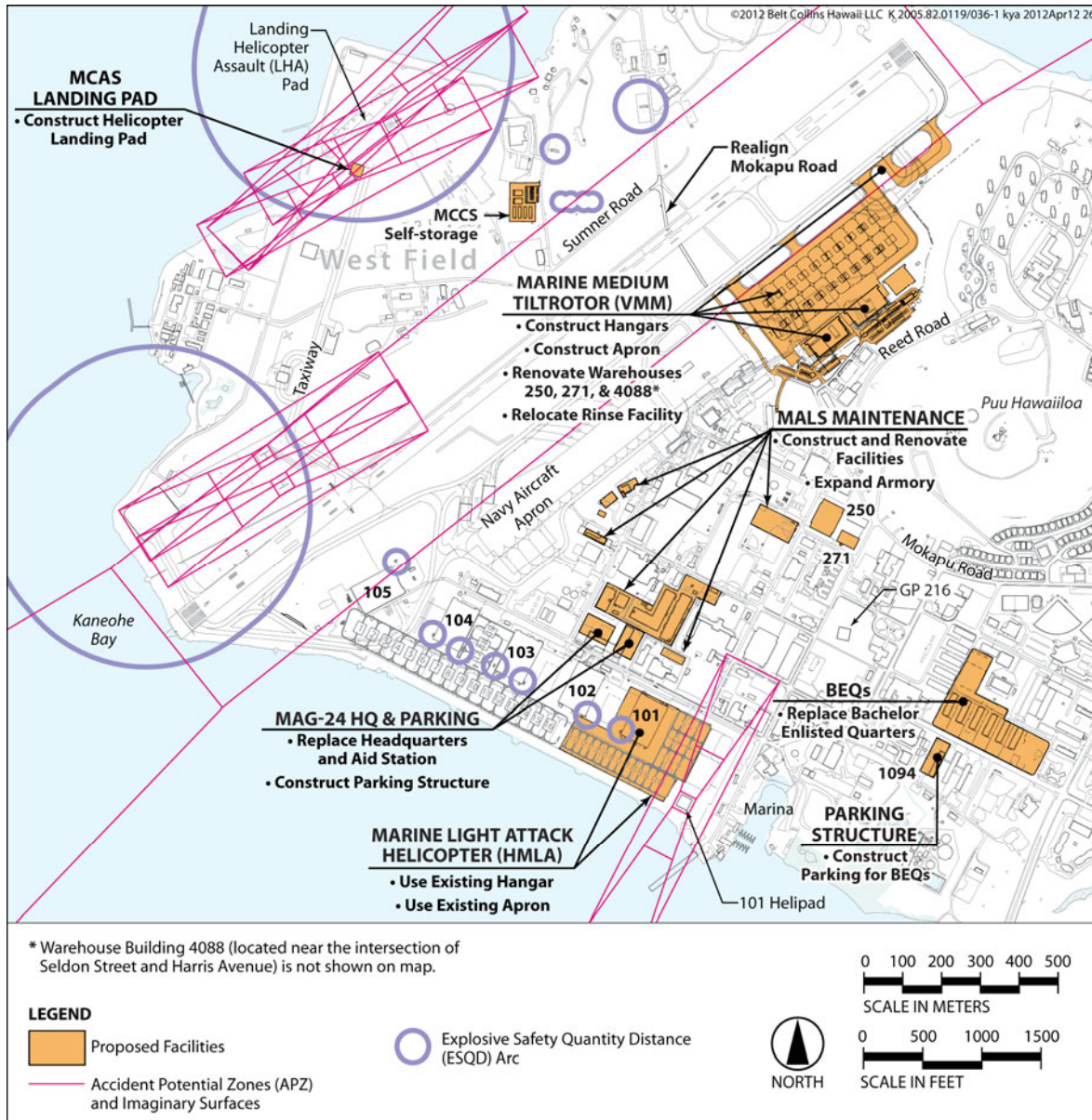
Figure 2-3. Alternative A –Overview, MCB Hawaii Kaneohe Bay
