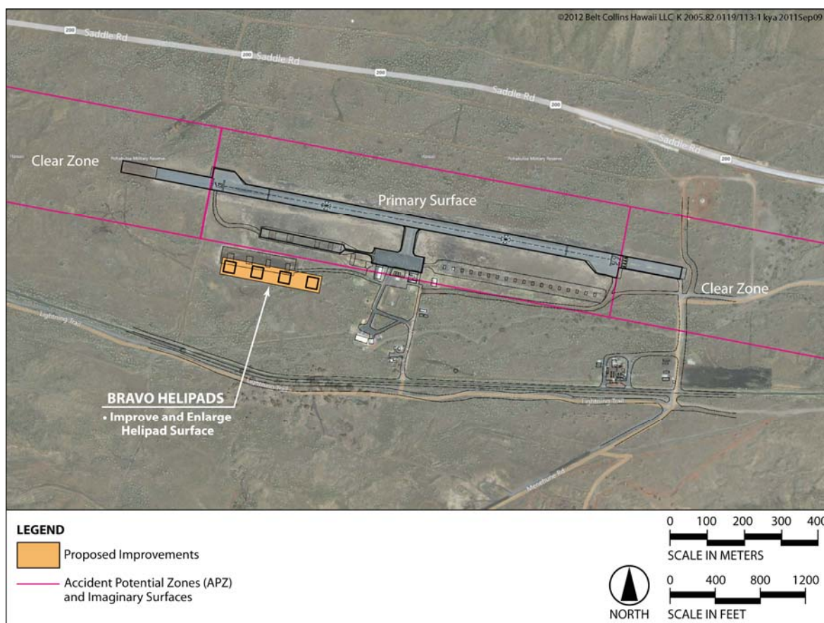
Figure 2-14. Bradshaw Army Airfield Improvements
