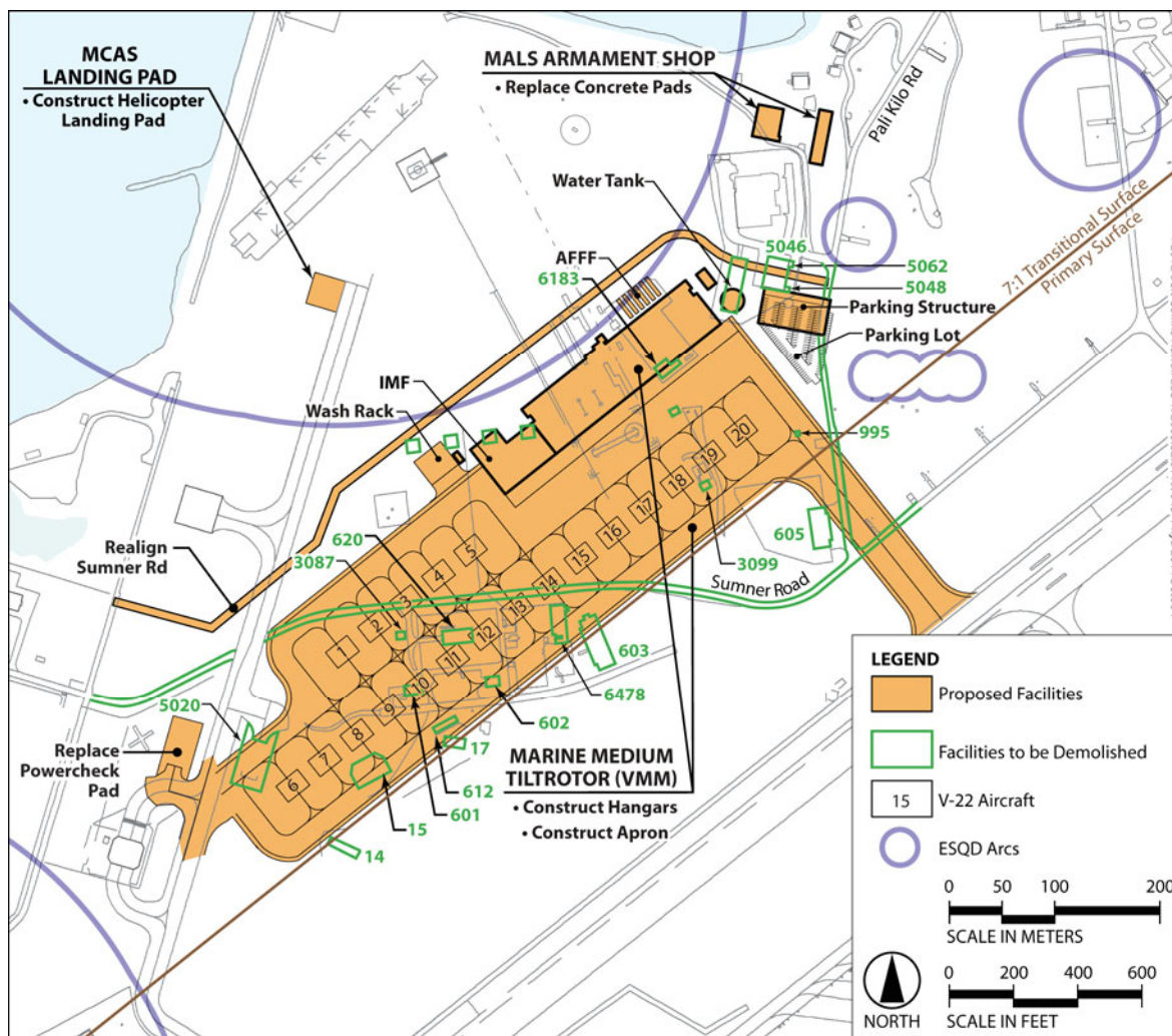
Figure 2-17. Alternative B—VMM Hangar and Apron, MCB Hawaii Kaneohe Bay
