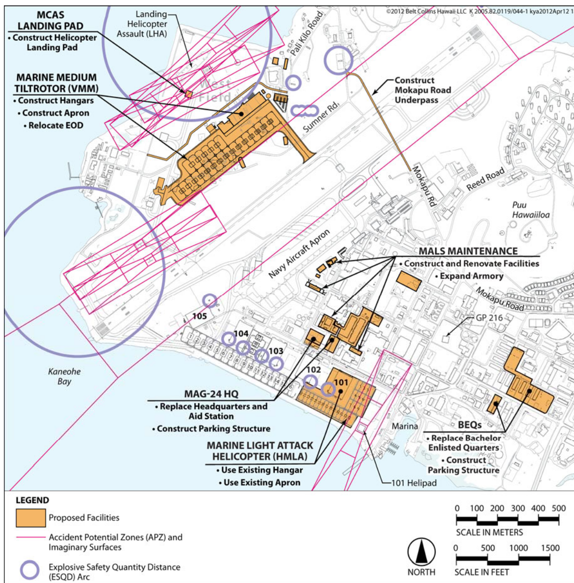
Figure 2-16. Alternative B—Overview, MCB Hawaii Kaneohe Bay
