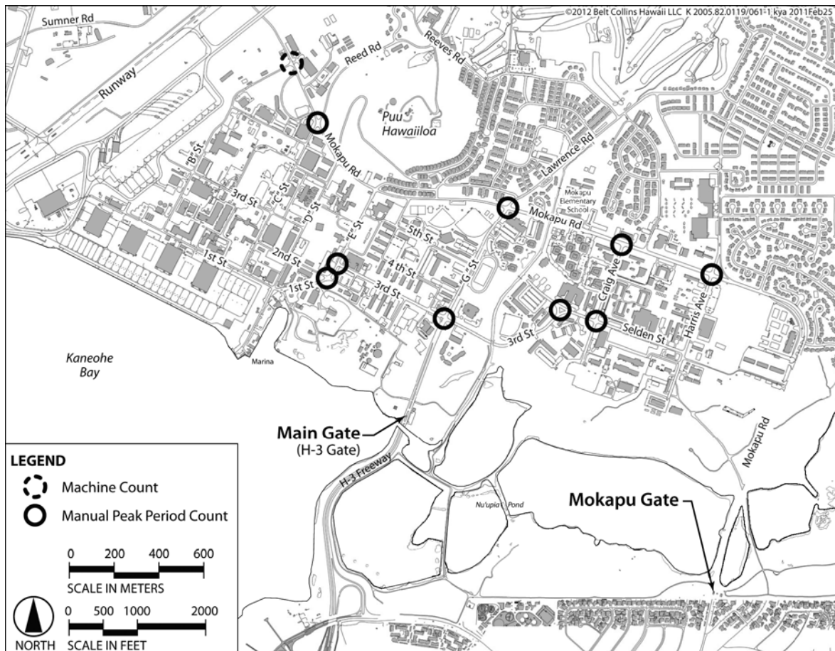
Figure 3-16. Traffic Count Locations
