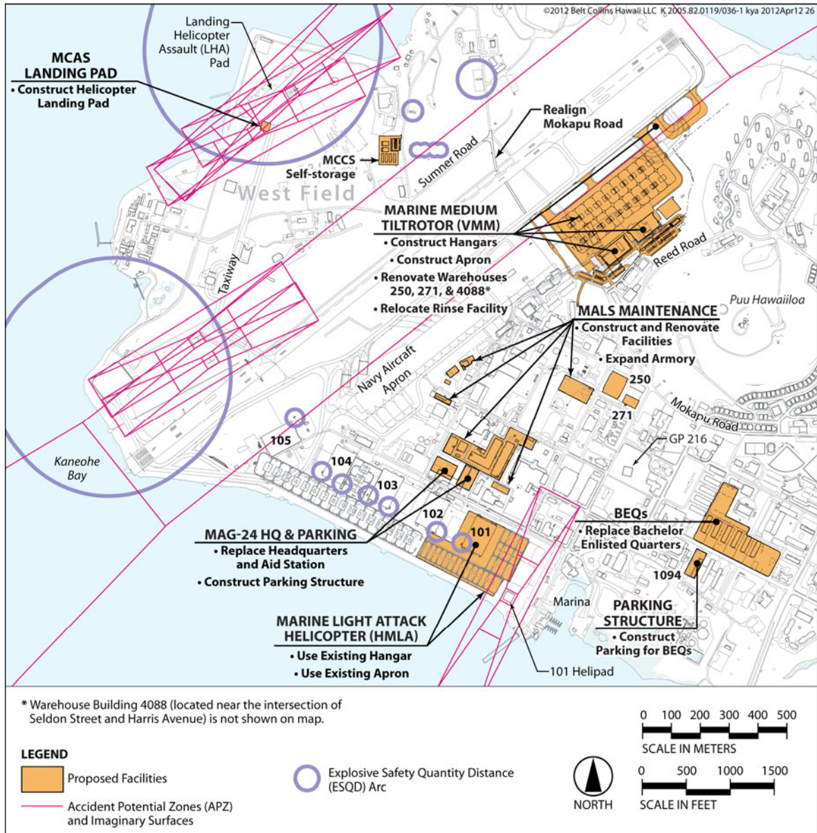
Figure ES-1. Alternative A – Overview, MCB Hawaii Kaneohe Bay
